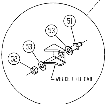
STRIKER BOLT DETAIL 4X SCALE
