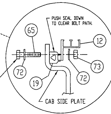
TYPICAL BOTTOM EDGE BOLTING PATTERN 5X SCALE
