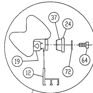
WINDOW CLAMP INSTALL 5X SCALE
